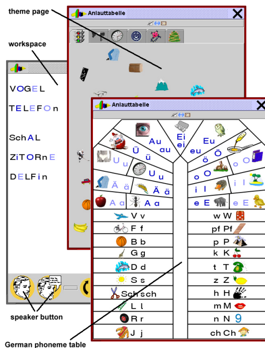
Fig. 3: Main parts of T 3 's user interface. The German phoneme table on the right side (uses different colours for consonants, short and long vowels), a page of prepared words together with their visual representation, and the child's result (most of the words are already phonetically correctly spelt) in the writing board on the left.
