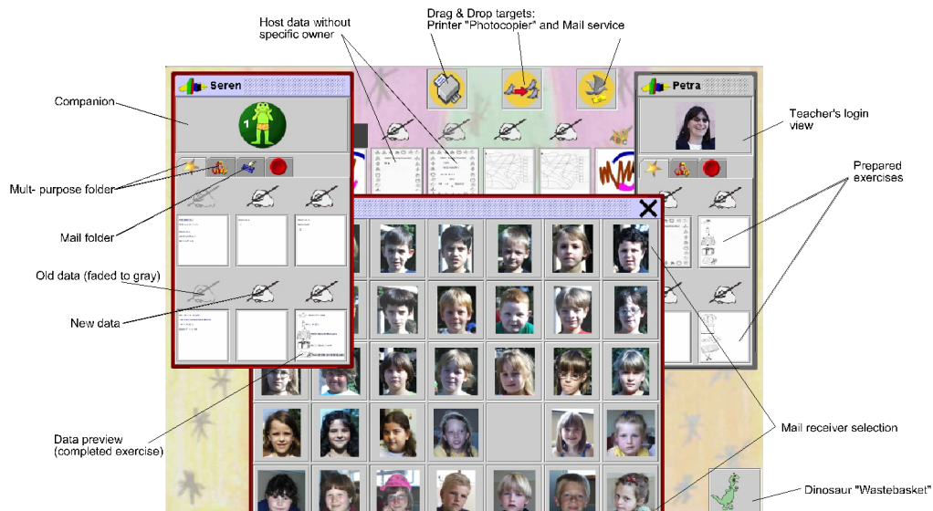
Fig. 2: Elements of the NIMIS Desktop
